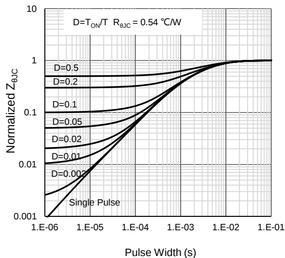
Figure 19: Normalized Maximum Diode Transient Thermal Impedance
