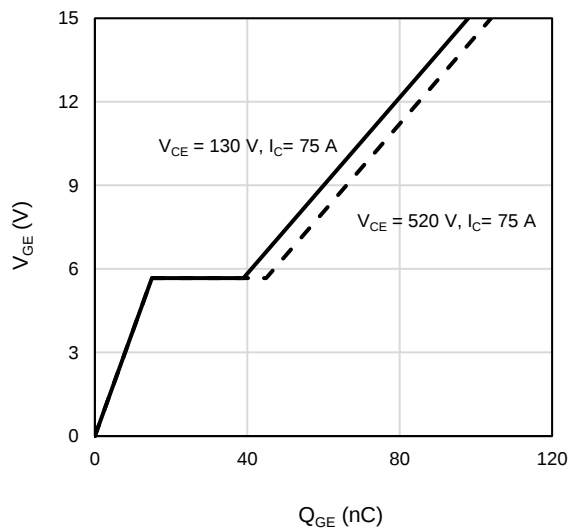
Figure 16: Gate-Charge Characteristics
