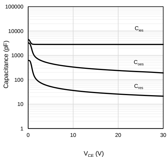
Figure 17: Capacitance Characteristics
